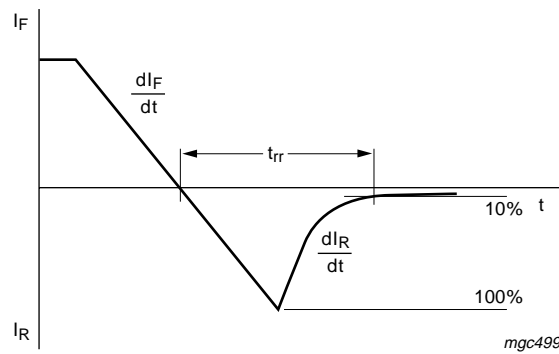
Fig 10. Test circuit and reverse recovery time waveform and definition
